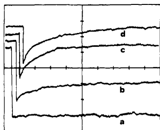
Figure 4. Transmission changes ( \lambda 412 nm) after pulse irradiation (dose = 1.9 krad) of phosphate buffer ( 6.2 \times 10^{-3} M, pH 7.2)/2-propanol ( 6.5 M)/acetone ( 3.4 \times 10^{-3} M) solutions containing deuterohemin ( 10^{-4} M) and various carbon tetrachloride concentrations. Scales: vertical, \Delta T = 2\% /div; horizontal, time = 10 ms/div. Carbon tetrachloride concentration: (a) 0; (b) 0.25 \times 10^{-4} M; (c) 0.7 \times 10^{-4} M; (d) 10^{-4} M.
