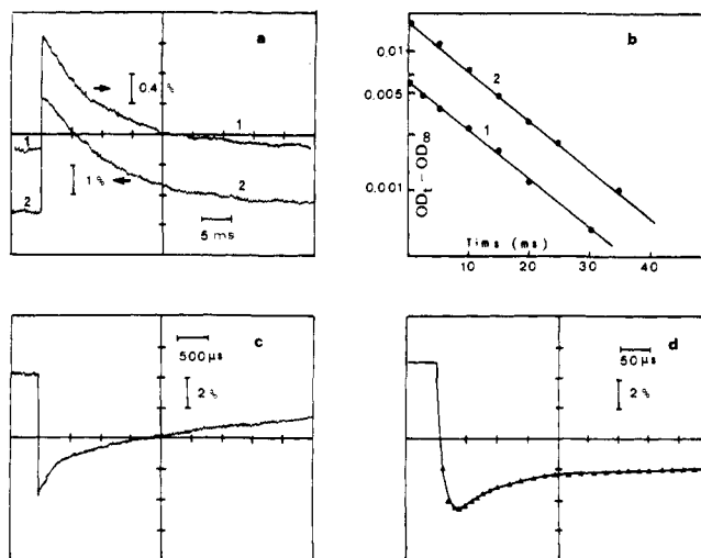
Figure 5. Transmission changes after pulse irradiation of phosphate buffer ( 6.2 \times 10^{-3} M, pH 7.2)/2-propanol ( 6.5 M)/acetone ( 3.4 \times 10^{-2} M) solutions containing deuterohemin ( 10^{-4} M) and carbon tetrachloride ( 10^{-4} M): (a) \lambda 387 nm, dose = 0.67 (1) and 2.2 krad (2); (b) same experiment, semilogarithmic plots of (\text{OD}_t - \text{OD}_\infty) vs. time; (c) \lambda 412 nm, dose = 5.8 krad; (d) \lambda 412 nm, dose = 6.2 krad. \blacktriangle , experimental; —, theoretical curve calculated with k_{13} = 2 \times 10^9 \text{ M}^{-1} \text{ s}^{-1} (see text).
