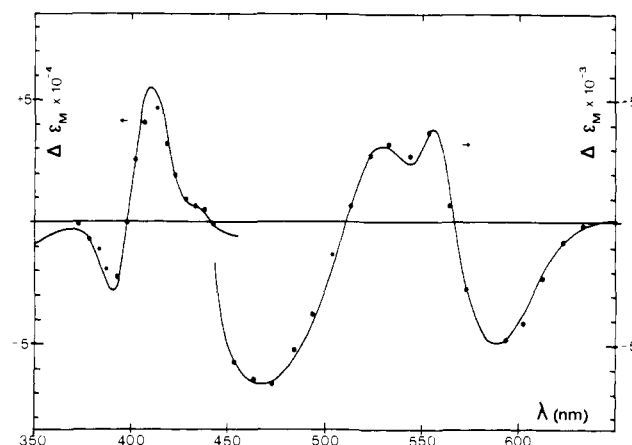
Figure 3. Reduction of deuterohemin by \alpha -hydroxyisopropyl radicals. Solvent phosphate buffer ( 6.2 \times 10^{-3} M, pH 7.2)/2-propanol ( 6.5 M)/acetone ( 3.4 \times 10^{-2} M). Difference spectra ( \text{DPFe}^{\text{II}} minus \text{DPFe}^{\text{III}} ) obtained from conventional reduction methods (—) and from pulse radiolysis study (●).
