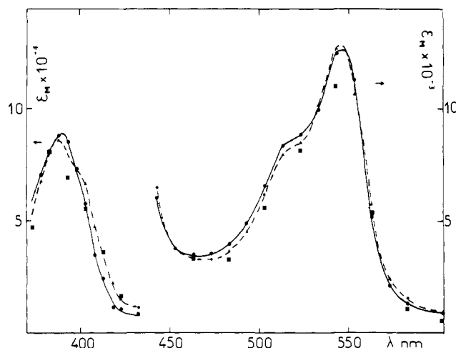
Figure 6. Reconstituted visible and near-UV spectra of transient species formed after pulse radiolysis of 10^{-4} \text{ M} deuteroheme in phosphate buffer ( 6.2 \times 10^{-3} \text{ M} , pH 7.2)/2-propanol (6.5 M) mixture containing sodium dithionite ( 10^{-4} \text{ M} ) and dichloromethane ( 4 \times 10^{-2} \text{ M} ): —, 100 \mu\text{s} after the pulse ( \bullet , experimental points); --, 4.5 ms after the pulse ( \blacktriangle , experimental points). \blacksquare , Visible and near-UV spectra of the transient species observed 4.5 ms after pulse radiolysis of 10^{-4} \text{ M} deuterohemin in phosphate buffer ( 6.2 \times 10^{-3} \text{ M} , pH 7.2)/2-propanol (6.5 M) mixture containing dichloromethane ( 4 \times 10^{-2} \text{ M} ). The dose is 1.4 krad in both cases.
