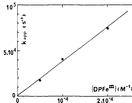
Figure 2. Reduction of deuterohemin by \alpha -hydroxyisopropyl radicals. Solvent phosphate buffer ( 6.2 \times 10^{-3} M, pH 7.2)/2-propanol ( 6.5 M)/acetone ( 3.4 \times 10^{-2} M). Plot of k_{\text{app}} vs. deuterohemin concentration.
