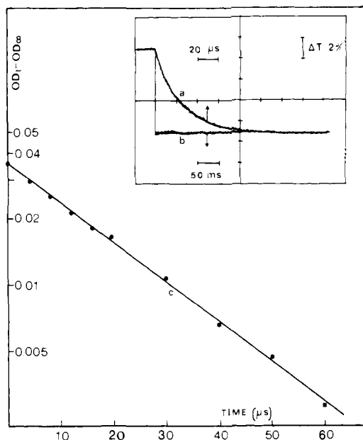
Figure 1. Reduction of deuterohemin by \alpha -hydroxyisopropyl radicals. Solvent phosphate buffer ( 6.2 \times 10^{-3} M, pH 7.2)/2-propanol ( 6.5 M)/acetone ( 3.4 \times 10^{-2} M); deuterohemin concentration 10^{-4} M; dose 1.7 krad. (a, b) Transmission changes ( \lambda 407 nm). (c) Semilogarithmic plot of (OD_t - OD_\infty) vs. time.
